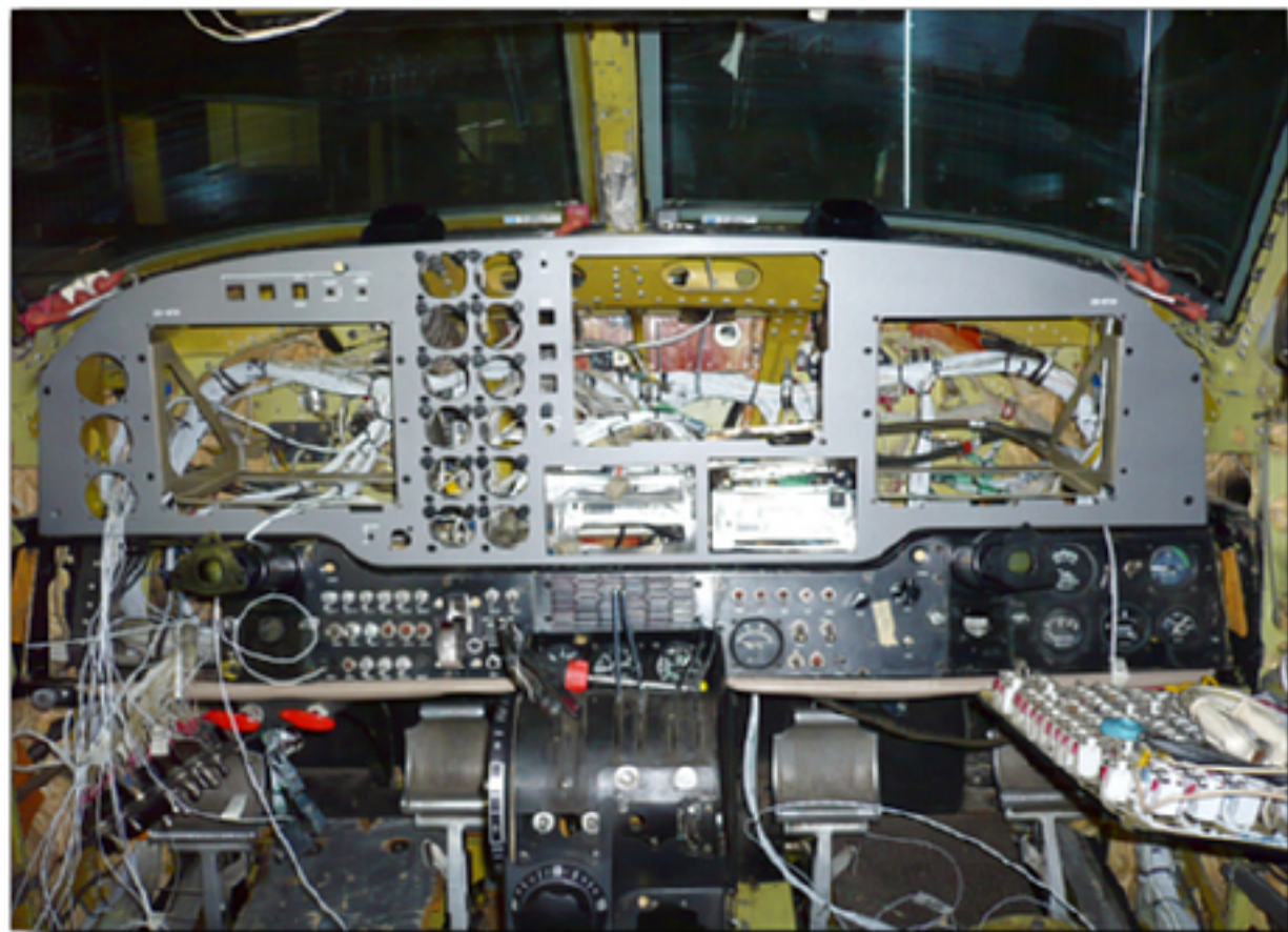
New instrument panel installed
